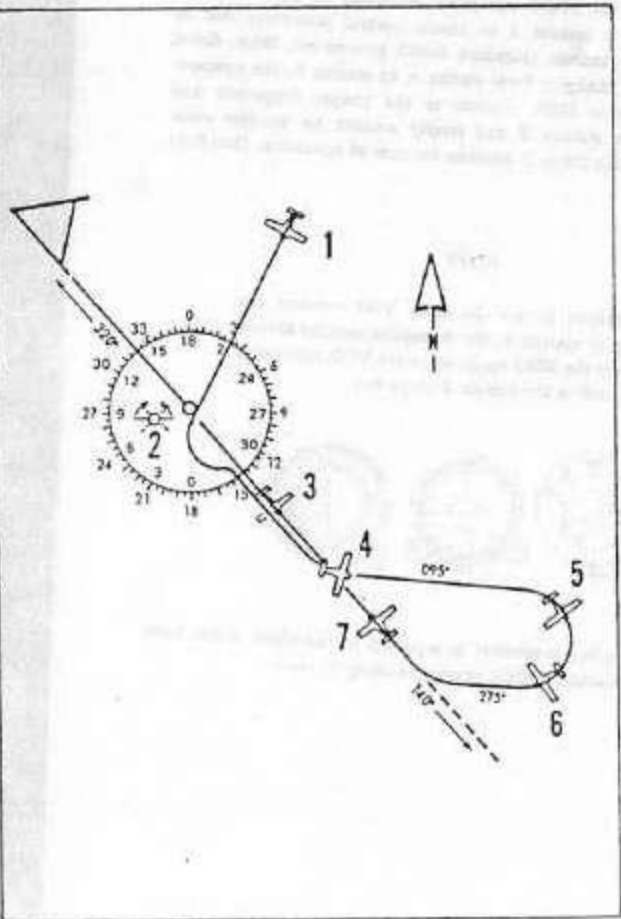
OMNI APPROACH
